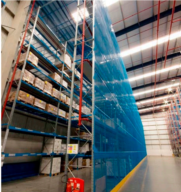
The Axelent SafeStore anti-collapse protection system is supplied with special brackets in customer-specific colours to match the rest of the customer's facility.
